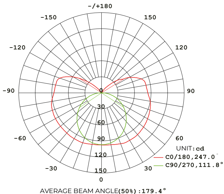
Light distribution
